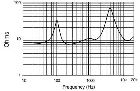
VR62 Impedance vs Frequency
