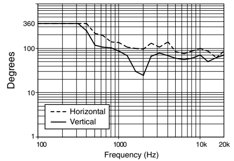
VR62 Beamwidth vs Frequency
